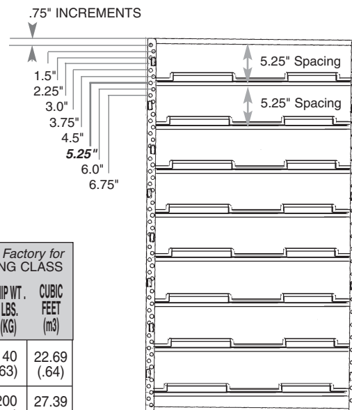
Side View of ETC-1240-10
