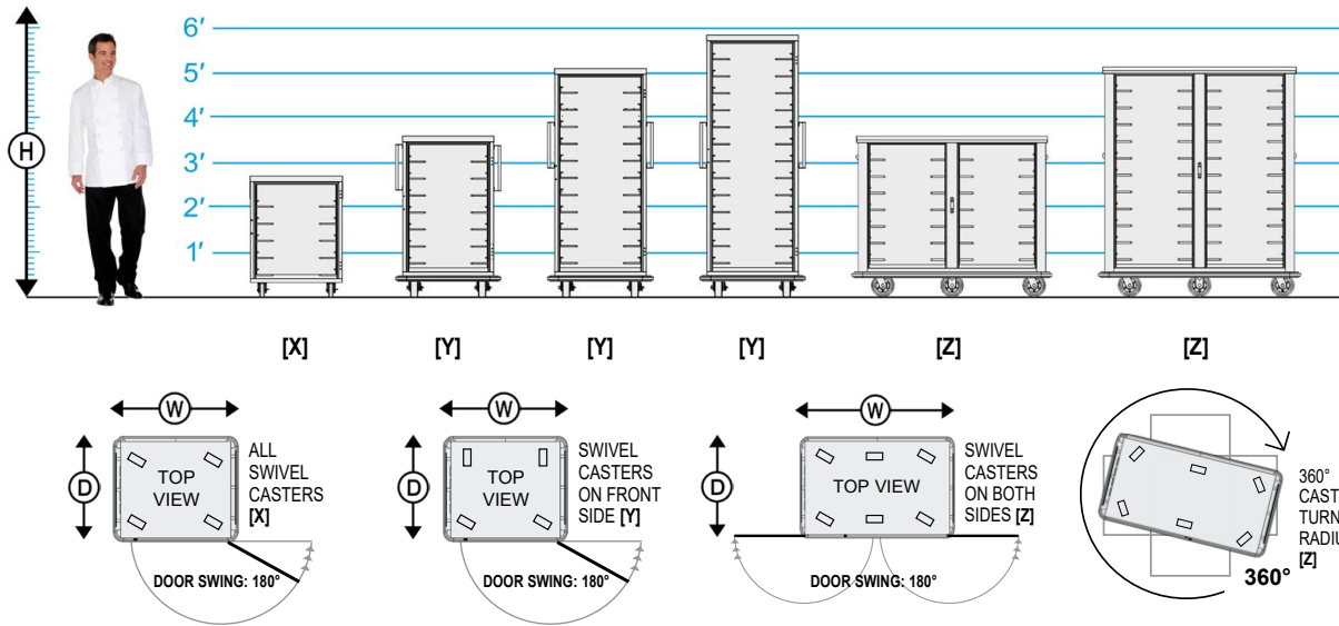
CAPACITIES OF TRAYS / PANS: 4.5" (114 mm) Spacings are Standard [A]
